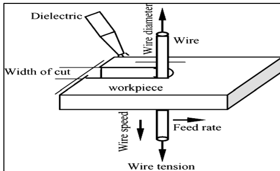
Fig 1: Wire-EDM Process [6]
